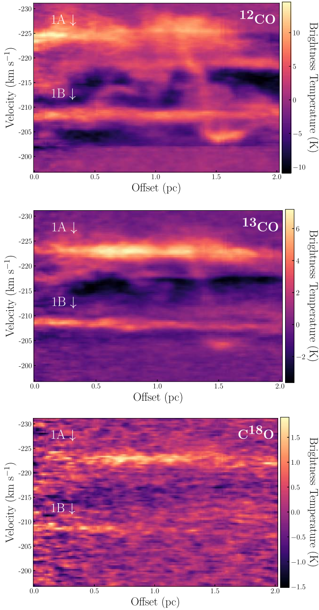
Figure 8. The filament 1 p-v diagrams for 12 CO (top), 13 CO (middle), and C 18 O (bottom), respectively. The p-v slice starts at the end of the filament that is closer to the Galactic center, so the offset represents the distance along the p-v slice as we move from left to right along the filament 1 spine (see Figure 5).
