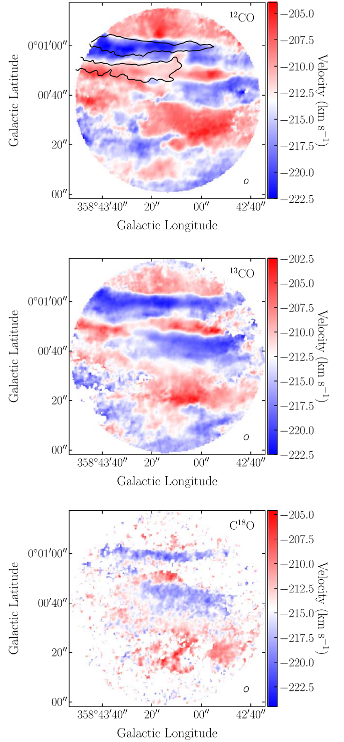
Figure 6. Spatially masked moment 1 maps generated from data subcubes in the velocity range of -197 \text{ km s}^{-1} to -231 \text{ km s}^{-1} for ^{12}\text{CO} , ^{13}\text{CO} , and \text{C}^{18}\text{O} , respectively. In the ^{12}\text{CO} image, the black contours indicate the filament 1 and filament 2 regions. For each image, the beam is indicated in the lower right corner.
