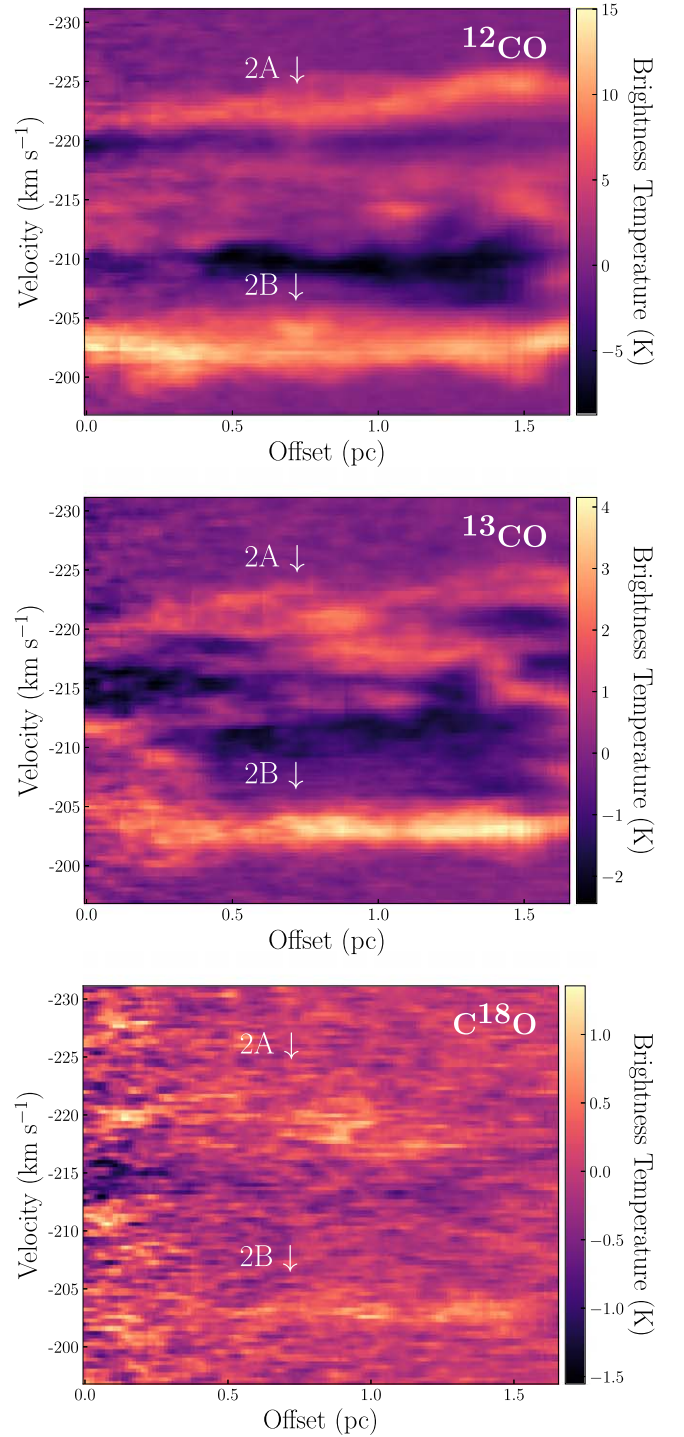
Figure 9. The filament 2 p-v diagrams for 12 CO (top), 13 CO (middle), and C 18 O (bottom), respectively. The p-v slice starts at the end of the filament that is closer to the Galactic center, so the offset represents the distance along the p-v slice as we move from left to right along the filament 2 spine (see Figure 5).
