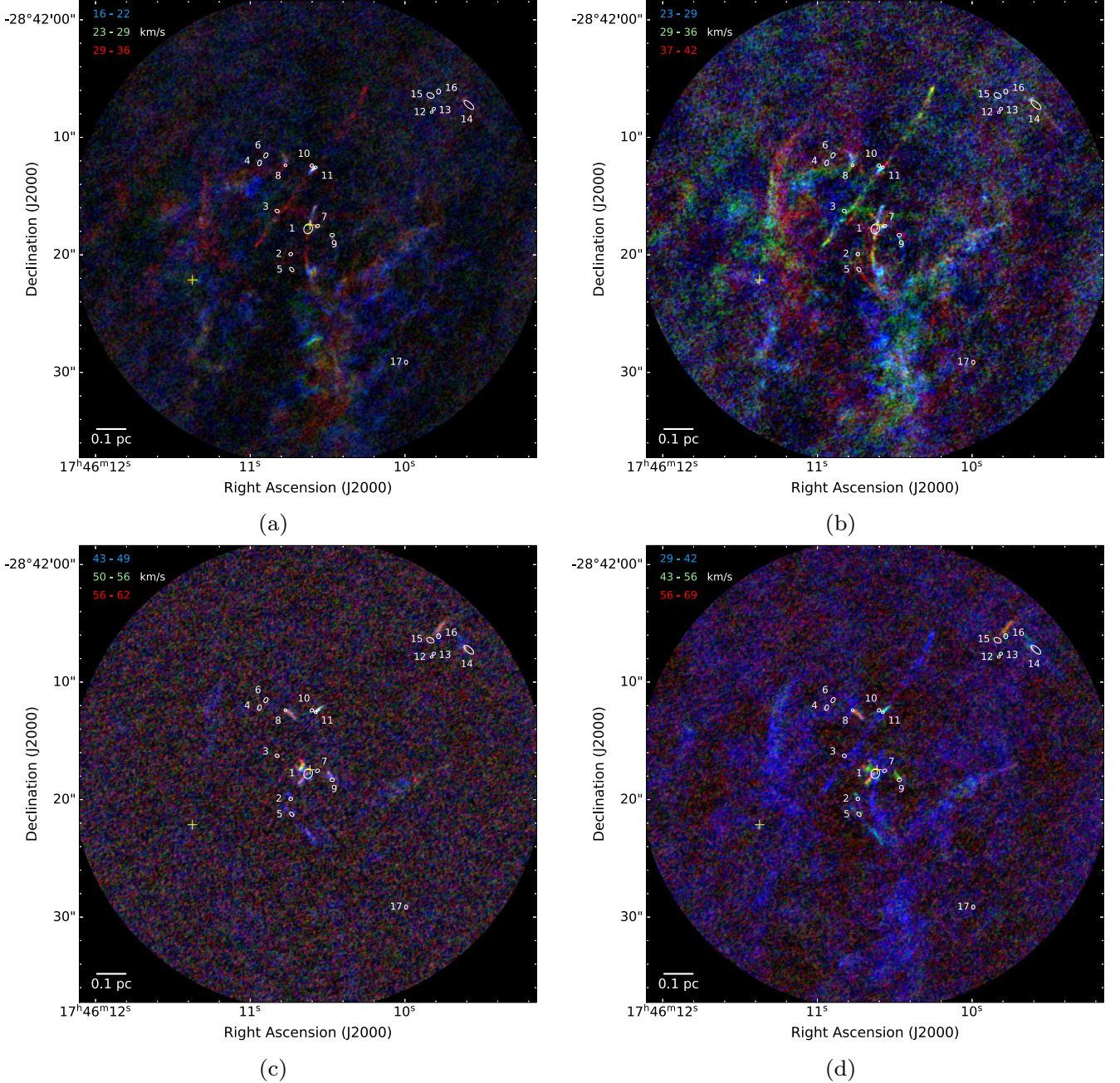
Figure 9. Three-colour figures showing the SiO (5–4) emission at different velocities. (a) 16–22 (blue), 23–29 (green), and 29–36 (red) \text{km s}^{-1} ; (b) 23–29 (blue), 29–36 (green), and 37–42 (red) \text{km s}^{-1} ; (c) 43–49 (blue), 50–56 (green), and 56–62 (red) \text{km s}^{-1} ; (d) 29–42 (blue), 43–56 (green), and 56–69 (red) \text{km s}^{-1} . Continuum sources are highlighted by white ellipses, the extent of which corresponds to the structures determined using dendrograms. Each continuum source is also numbered. The yellow crosses show the position of water masers from Lu et al. (2019b).
