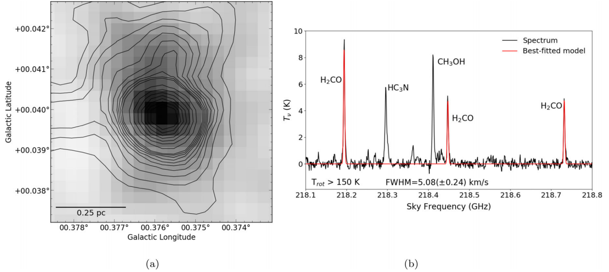
Figure A2. (a) Integrated intensity map of the para-H 2 CO 3 0,3 -2 0,2 transition towards ‘c1’. Black contours are SMA dust continuum. (b) Spatially averaged spectrum of the para-H 2 CO lines (plus HC 3 N and CH 3 OH). Using an LTE line-fitting routine, we fit the H 2 CO lines. Due to the large line ratios, we are unable to obtain a reliable gas temperature (see Fig. A1). We therefore provide a lower limit of 150 K, above which our temperature diagnostic is uncertain.
