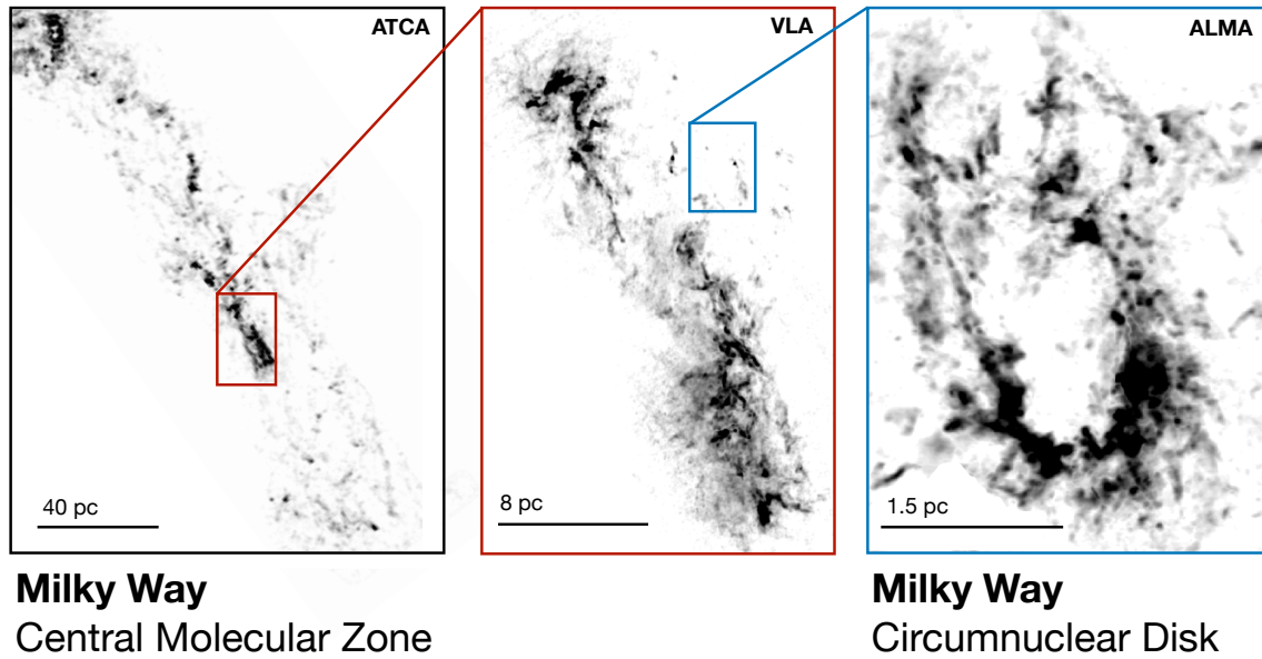
Fig. 1.— An illustration of the data sets to be used in order to probe the variation in physical properties with radius and size scale in the GC. Left: SWAG data showing ammonia emission from the entire central 200 pc of the GC. Center: VLA data (PI: Mills) showing ammonia emission from a single molecular cloud complex in the GC. Right: ALMA data showing HCN emission from the molecular gas surrounding the central supermassive black hole in the GC. Using these data, we will measure how temperature, turbulence, and density vary on sub-cloud scales, and how these properties vary with distance from the black hole and depth into the GC potential.
