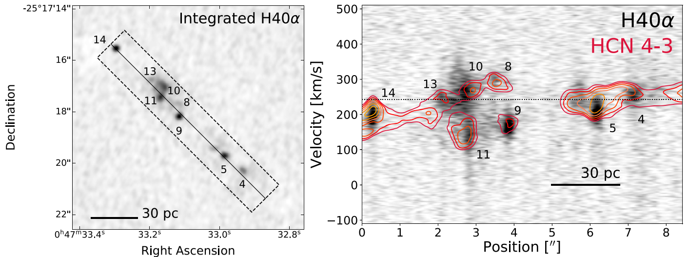
Figure 8. Left: map of integrated H \alpha emission showing the orientation and width of the slit used to extract a PV diagram. Right: PV diagram of H40 \alpha emission (gray scale) compared to HCN 4–3 emission (red contours) along the same slit. The horizontal dotted line shows the rest-frame velocity of NGC 253. Emission at large positive velocities is seen between sources 10 and 13 in H40 \alpha but not in HCN 4–3. While there also appears to be large negative-velocity emission extending away from many of the sources (e.g., 4, 5, 9, 11, 13), this is contaminated by the presence of He40 \alpha emission.
