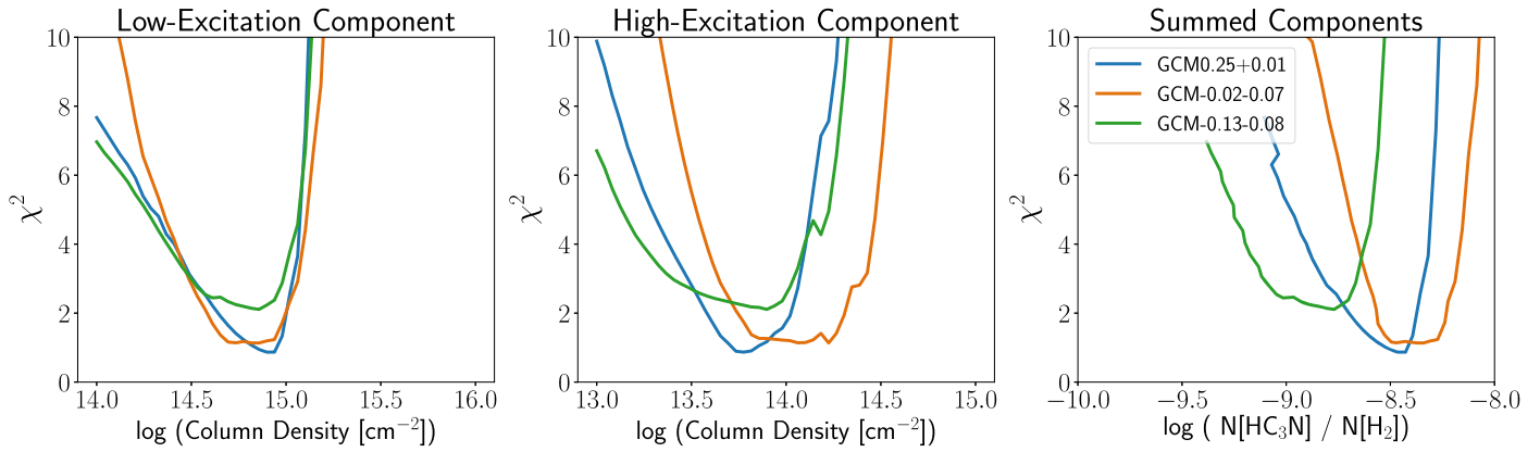
Figure 7. Chi-squared values for the column density of the low- and high-excitation components (left and middle) for each of the three observed clouds, GCM 0.25 +0.01, GCM -0.02–0.07, and GCM -0.13–0.08, marginalized over all other parameters. On the right, we show the best-fit abundance from summing the best-fit column densities and comparing to the average Herschel -derived \text{H}_2 column densities extracted from the same apertures as the \text{HC}_3\text{N} spectra.
