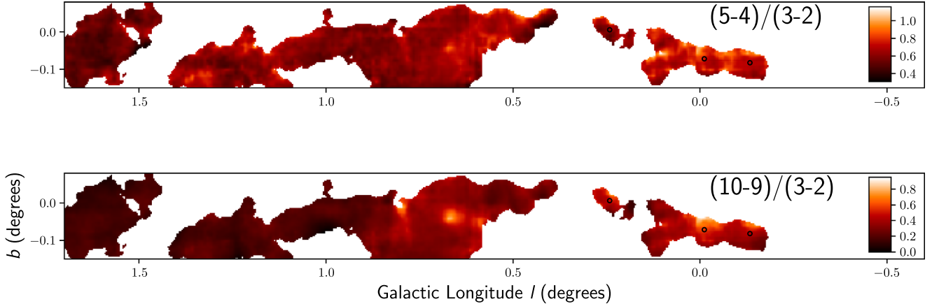
Figure 4. Ratio maps of the \text{HC}_3\text{N} J = (5-4) to (3-2) lines (top) and J = (10-9) to (3-2) lines (bottom). As in Figure 1, circles indicate the positions of pointed observations made with the GBT. A qualitative difference between the inner CMZ (right half) and the 100 \text{ pc} < r < 200 \text{ pc} region (left half) is evident: the excitation is lower beyond the orbit of Sgr B2. This difference suggests that the gas in the outer CMZ has a lower average density and/or lacks a high-density (high-excitation) component, consistent with models in which the CMZ is fed by highly turbulent, non-star-forming gas driven in by the Galactic bar.
