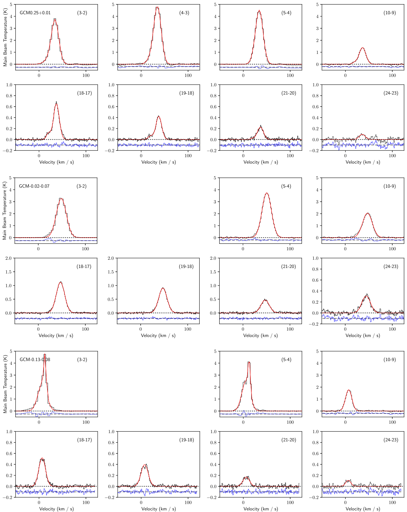
Figure 2. Spectra of \text{HC}_3\text{N} in the GCM 0.25+0.01 cloud (top), the GCM -0.02-0.07 cloud (middle), and the GCM -0.13-0.08 cloud (bottom). Gaussian fits to each line are overplotted in red, and the residuals of the fits are plotted below the spectrum in blue.
