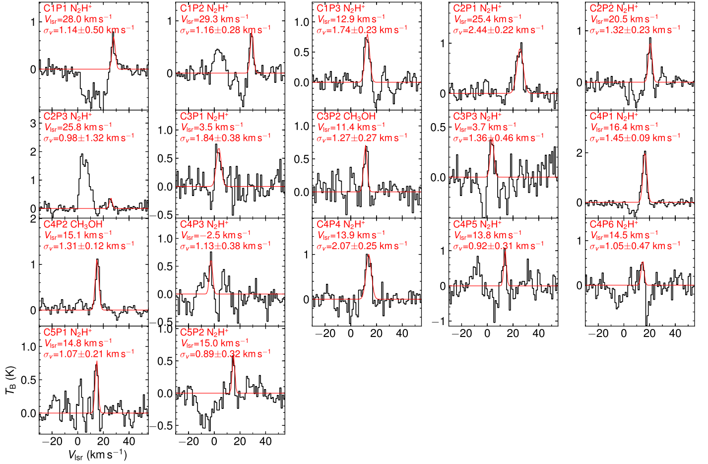
Figure 14. SMA \text{N}_2\text{H}^+ or \text{CH}_3\text{OH} spectra and best-fit models of cores in the 20 \text{ km s}^{-1} cloud. The best-fit centroid velocities ( V_{\text{LSR}} ) and line widths ( \sigma_v , deconvolved from channel width) are noted in each panel.
