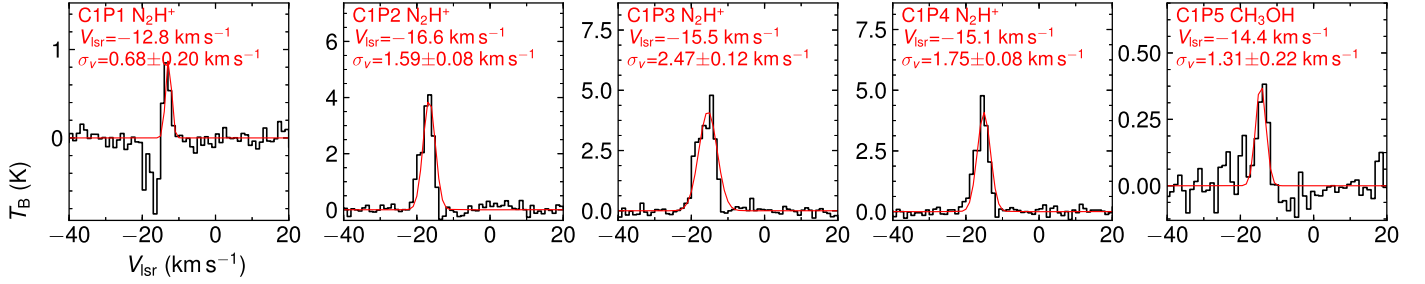
Figure 19. SMA N 2 H + or CH 3 OH spectra and best-fit models of cores in Sgr D. The best-fit line widths (deconvolved from channel width) are noted in each panel.
