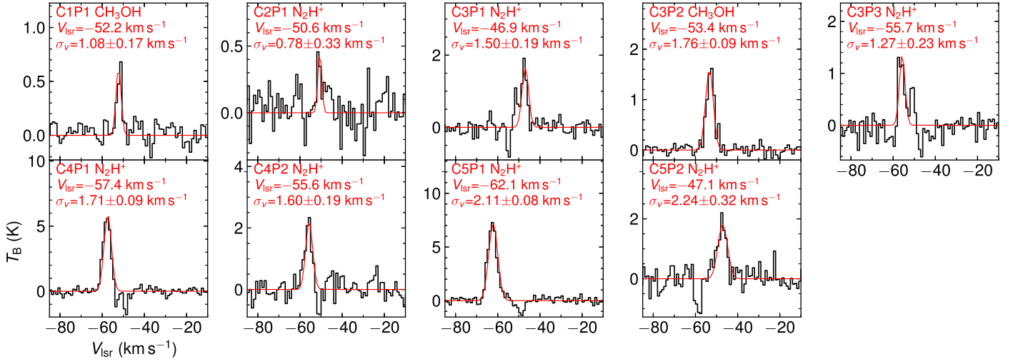
Figure 18. SMA N 2 H + or CH 3 OH spectra and best-fit models of cores in Sgr C. The best-fit line widths (deconvolved from channel width) are noted in each panel.
