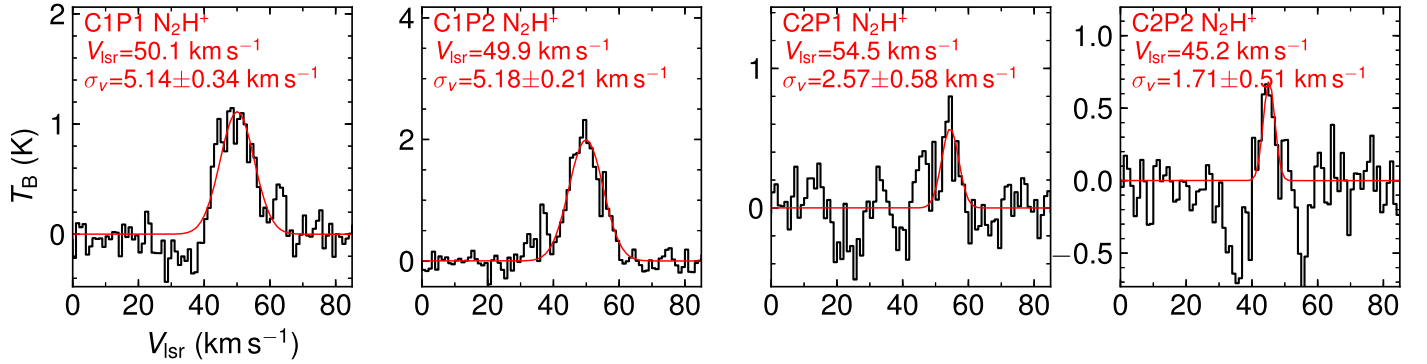
Figure 15. SMA \text{N}_2\text{H}^+ spectra and best-fit models of cores in the 50 \text{ km s}^{-1} cloud. The best-fit line widths (deconvolved from channel width) are noted in each panel.
