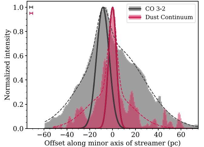
Figure 3. The normalized width profiles of the SW streamer, where the streamer has been summed along its major axis. The shaded histograms show the width profiles for the dust continuum (red) and CO 3–2 (gray). For the CO, this profile is the integrated intensity over the velocity channels shown in Figure 4. These profiles are fit with a two-component Gaussian, shown as the dashed curves. The narrow components (corresponding to the outflow) of the fits are shown as the solid curves, where the respective beam sizes have been deconvolved. The FWHM beam sizes are shown in the upper-left corner. The x -axis is the offset along the minor axis of the streamers relative to the centroid of the narrow dust component. The dust continuum component of the SW streamer is intrinsically narrower than and offset from the CO 3–2.
