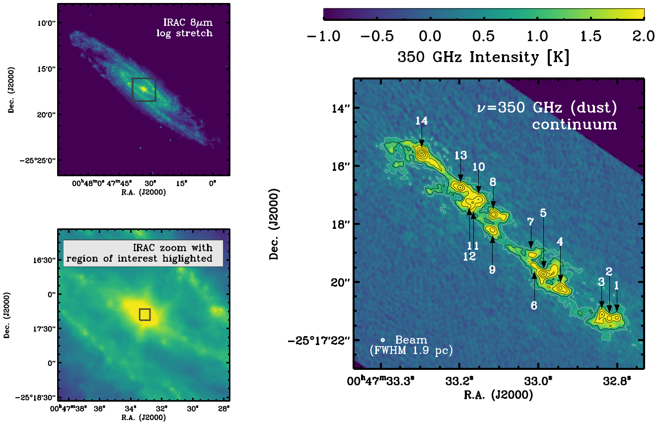
Figure 1. (Top left) Local Volume Legacy IRAC 8 \mu\text{m} image of NGC 253 (Dale et al. 2009; Lee et al. 2009). The square shows the region highlighted in the bottom left panel. (Bottom left) The field analyzed in this article (square box) plotted over the central part of the 8 \mu\text{m} image. We focus on the innermost region of the galaxy. This region hosts \sim 10 dense molecular clouds (e.g., Sakamoto et al. 2011; Leroy et al. 2015; Ando et al. 2017) and a large amount of high-density gas (e.g., Paglione et al. 2001; Knudsen et al. 2007; Leroy et al. 2015; Meier et al. 2015) and forms stars at a rate of \approx 2 M_{\odot} \text{ yr}^{-1} (see Bendo et al. 2015; Leroy et al. 2015). (Right) ALMA \nu = 350 GHz continuum emission from the inner region of NGC 253 at 0''.11 \sim 1.9 pc resolution. The emission, which is mostly from dust at this frequency, shows 14 bright peaks, each only moderately extended relative to the 1.9 pc beam. The sizes, implied dust optical depths at \nu = 350 GHz ( \sim 850 \mu\text{m} ), kinematics, and association with dense, excited gas suggest that many of these peaks may represent forming SSCs (see Sections 3 and 4). Note that we show a 10'' \times 10'' cutout covering the region of interest, but that the FWHM of the primary beam of ALMA’s 12 m antennas is 18'' at 350 GHz. Contours in the continuum image show 0.6 K (gray), and 1, 2, 4, ... K (black).
