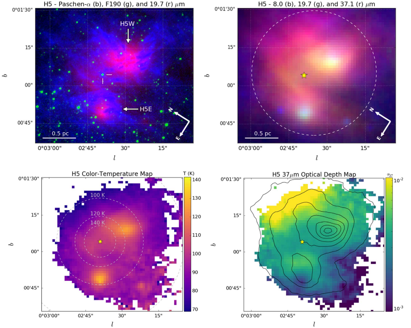
Figure 5. Top left: false-color image of H5 with HST Pa \alpha (blue), HST F190 (green), and SOFIA/FORCAST 19.7 \mu m (red). P107, the candidate ionizing source of H5, is visible in the F190 image and is indicated by the perpendicular white lines. The locations of the components H5E and H5W are also indicated. Top right: false-color image of H5 with Spitzer /IRAC 8 \mu m (blue), SOFIA/FORCAST 19.7 \mu m (green), and SOFIA/FORCAST 37.1 \mu m (red). The location of P114 is marked by a yellow star in this panel and the two bottom panels. The photometric extraction area is shown by the dashed circle. Bottom left: color-temperature map of H5 with contours (gray dashed) denoting equilibrium temperatures based on dust heating by P107; we suggest that this star is unlikely to be the heating source (see Section 4.4). Bottom right: 37 \mu m optical depth map of H5 with 37 \mu m contours (ranging from 0.2 to 1.4 in increments of 0.2 Jy pixel -1 ).
