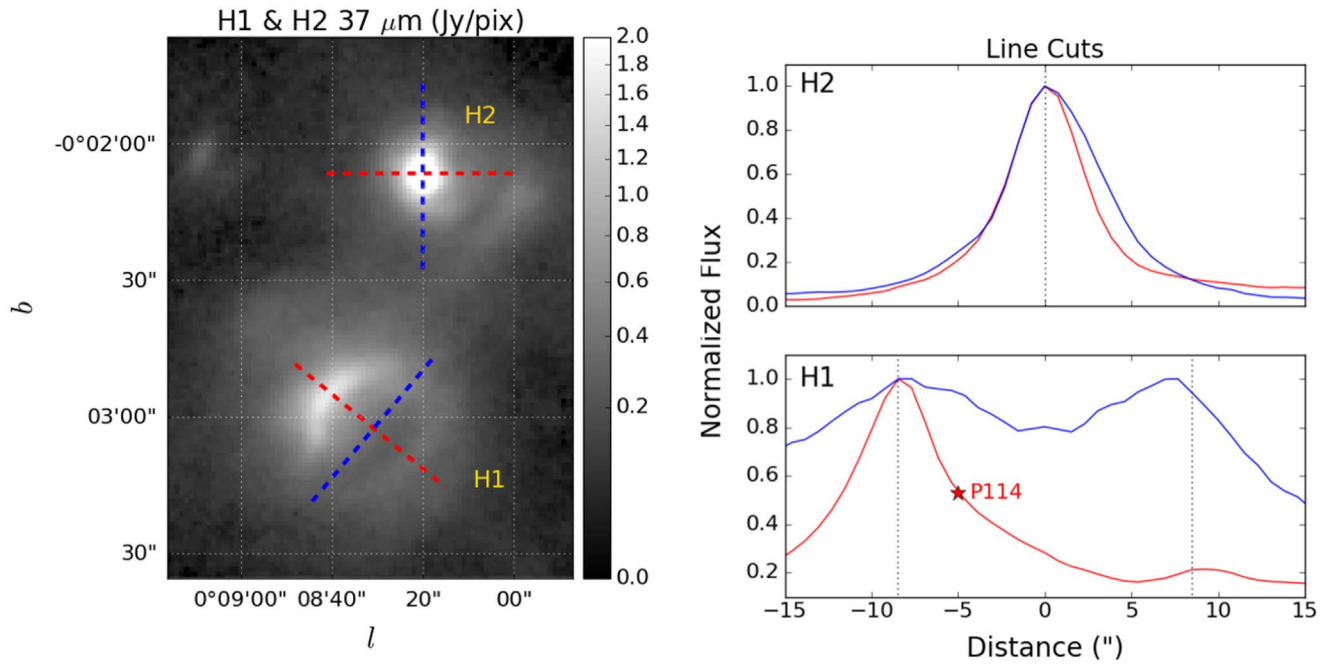
Figure 9. Line cuts through H1 and H2NE. H1 appears to have a bubble-like morphology at 37\ \mu\text{m} . The apparent continuation of the bright arc-like feature into a larger bubble suggests that the shape of H1 may be generated by a density gradient in the surrounding medium. The line cuts through H1 are centered on the apparent bubble, and the location of P114 is indicated with a red star. H2NE is resolved by FORCAST, although there is not any detailed structure present outside of the bright central peak, which corresponds to the location of P35.
