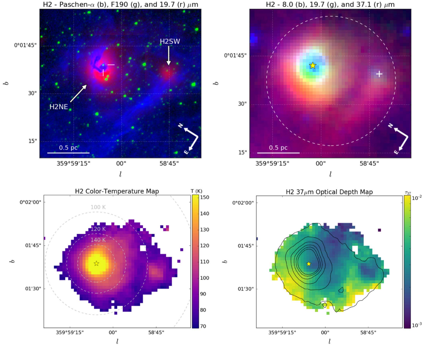
Figure 3. Top left: false-color image of H2 with HST Pa \alpha (blue), HST F190 (green), and SOFIA/FORCAST 19.7 \mu m (red). P35, the candidate ionizing source of H2, is visible in the F190 map, and its position is indicated by the white crosshairs. The locations of the two components H2NE and H2SW are also indicated. A scale bar and cardinal directions in equatorial coordinates are shown in the lower left and right corners, respectively. Top right: false-color image of H2 with Spitzer /IRAC 8 \mu m (blue), SOFIA/FORCAST 19.7 \mu m (green), and SOFIA/FORCAST 37.1 \mu m (red). The location of P114 is marked by a yellow star in this panel and the two bottom panels. The location of H2SW (19.7 \mu m centroid) is marked by the white plus sign, and the photometric extraction area is shown by the dashed circle. Bottom left: color-temperature map of H2 with contours (gray dashed) denoting equilibrium temperatures based on dust heating by P35. Bottom right: 37 \mu m optical depth map of H2 with 37 \mu m contours (ranging from 0.3 to 1.8 in increments of 0.3 Jy pixel -1 ). H2SW is not visible in the 37 \mu m contours because its emission is dominated by an extended dust filament.
