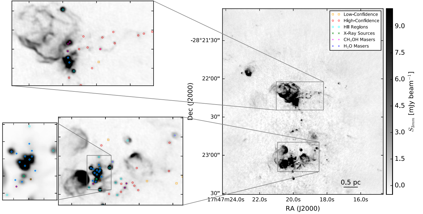
Figure 3. Close-in look at the Sgr B2 M and N region. Multiple insets show identified sources in some of the richer subregions. The points are colored as in Figure 2. The background image is the ALMA 3 mm continuum. See also Figure 22.
