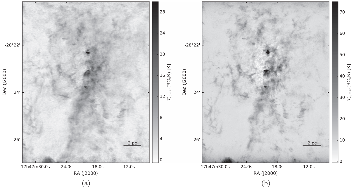
Figure 21. Peak-intensity maps of \text{HC}_3\text{NJ} = 10\text{--}9 . The left panel shows the 12 m short-baseline data combined with 7 m and total power data; by excluding the long-baseline data, the large angular scales are emphasized. The right panel shows the robust 0.5-weighted 12 m+7 m data combined with total power data; it reaches a substantially higher peak intensity in the compact regions, but the lower-intensity diffuse emission is relatively hidden. In the right panel, the negative bowls seen near Sgr B2 M and N in this peak-intensity image indicate that intermediate size scales were not well recovered. The bright feature on the lower left of both images may be an imaging artifact.
