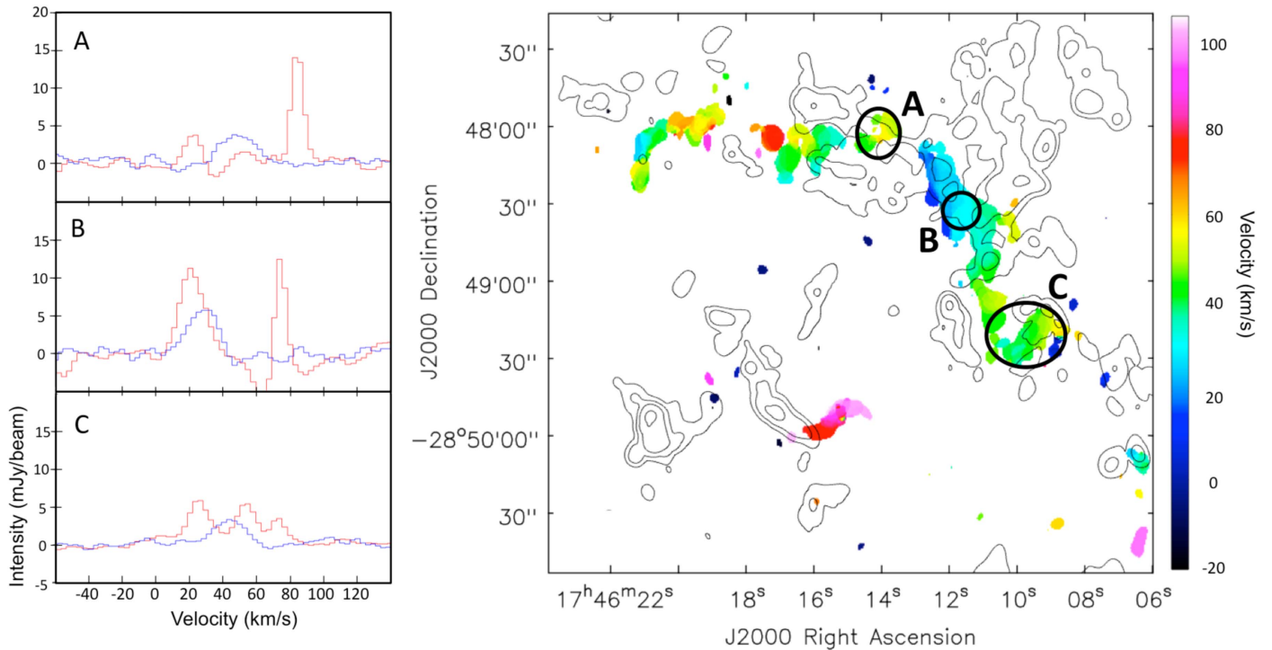
Figure 5. (Left): spectra of both the molecular (red: \text{NH}_3 (3, 3)) and ionized (blue: \text{H63}\alpha + \text{H64}\alpha ) gas toward the Sickle H II region. (Right): color scale shows the intensity-weighted velocity distribution of the combined \text{H63}\alpha + \text{H64}\alpha radio recombination lines over -20 – 100 \text{km s}^{-1} , with black contours of the \text{NH}_3 (3, 3) emission at 5, 10, 20, and 50 \times 3 \text{mJy beam}^{-1} . The contours and color scale in right are from Figure 4, top left and bottom right, respectively.
