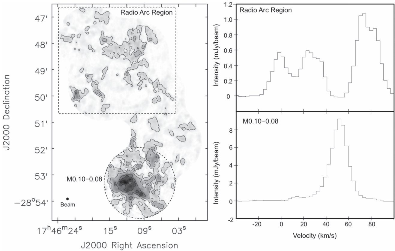
Figure 3. (Left): maximum intensity \text{NH}_3 (3, 3) emission ( 5''.0 \times 5''.0 , PA = 0^\circ , resolution), integrated over a velocity range of -20 – 100 \text{km s}^{-1} , with contours showing: 5, 15, 50, 100, and 200 \times 3 \text{mJy beam}^{-1} (rms noise). (Right): spectra integrated over the outlined regions shown on the left for the Radio Arc region (top) and M0.10–0.08 (bottom).
