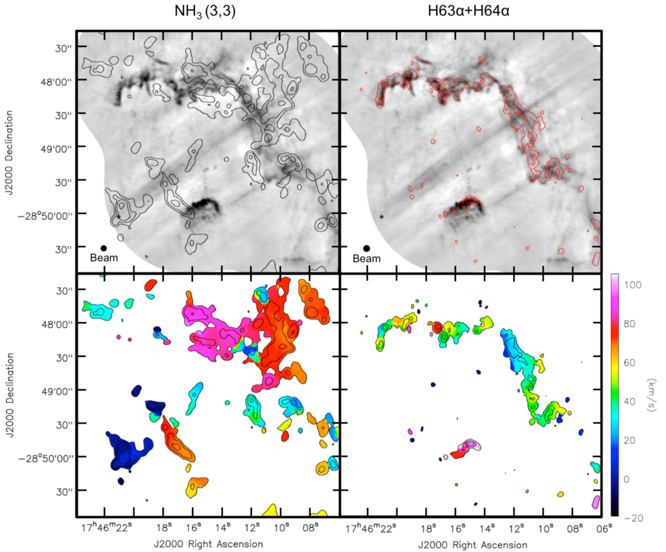
Figure 4. Distribution of \text{NH}_3 (3,3) ( 5''0 \times 5''0 , \text{PA} = 0^\circ , resolution, left panels) and combined \text{H63}\alpha + \text{H64}\alpha radio recombination lines ( 5''.68 \times 5''.61 , \text{PA} = 88.5^\circ , resolution, right panels). The top panels show maximum intensity contours in: \text{NH}_3 at 5, 10, 20, and 50 \times 3 \text{ mJy beam}^{-1} (rms level), and the combined \text{H63}\alpha + \text{H64}\alpha radio recombination lines at 5, 6, 8, and 10 \times 1.1 \text{ mJy beam}^{-1} (rms level) overlaid on the 24.5 GHz radio continuum, shown in grayscale. The bottom panels show the same maximum intensity contours, now overlaid on the intensity-weighted velocity distribution for emission between -20 and 100 \text{ km s}^{-1} .
