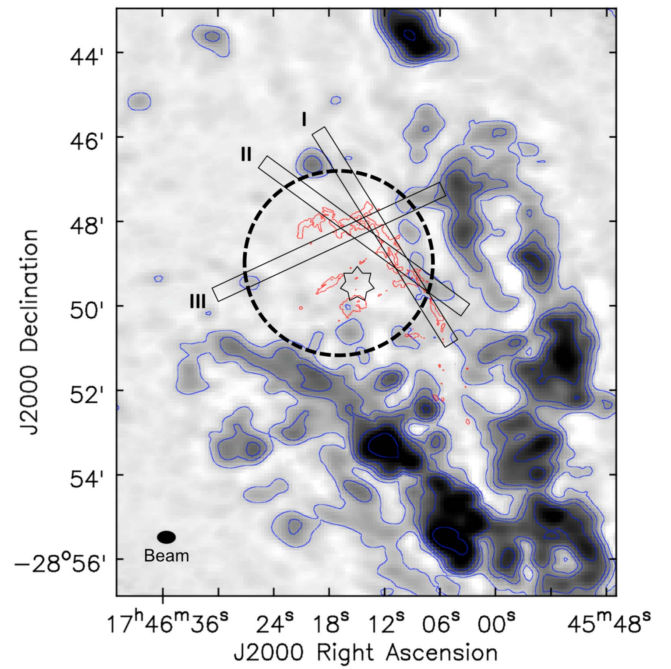
Figure 10. Maximum intensity \text{NH}_3 (3,3) emission from ATCA (SWAG survey; \sim 20'' resolution, bottom left corner; Ott et al. 2017) over a velocity range of 45\text{--}65 \text{ km s}^{-1} , with blue contours showing 5, 15, 25, 50 and 125 \times 20 \text{ mJy beam}^{-1} (rms level). The red contour represents the 24.5 GHz continuum emission (from Figure 2) above 0.5 \text{ mJy beam}^{-1} ( 10\sigma level). The black dashed circle shows the proposed size and location of the M0.20–0.033 expanding shell (see Figure 9 and Section 5.2.1). The star shows the location of the Quintuplet cluster. The black boxes show the relative lengths ( 350'' ) and integrated widths ( 5'' ) of slices I–III in Figure 11.
