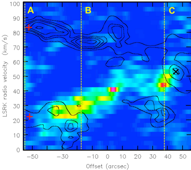
Figure 6. Position–velocity comparison of the ionized gas (color scale: \text{H63}\alpha + \text{H64}\alpha ; width = 18'' ) and the molecular gas (black contours: \text{NH}_3 ; width = 41'' ) from 17^{\text{h}}46^{\text{m}}12^{\text{s}}.9 , -28^{\circ}48'02''.7 ( -50'' offset) to 17^{\text{h}}46^{\text{m}}09^{\text{s}}.1 -28^{\circ}49'25''.8 ( +50'' offset). The spectral and spatial resolution for both transitions are \sim 3 \text{km s}^{-1} and \sim 5'' , respectively (see Section 2). The three yellow vertical dashed lines show the relative locations of the three regions in Figure 5. The red “+” signs mark the midpoint of the ellipse discussed in Section 5.2.2. The black “x” sign indicates the edge of ellipse, also discussed in Section 5.2.2.
