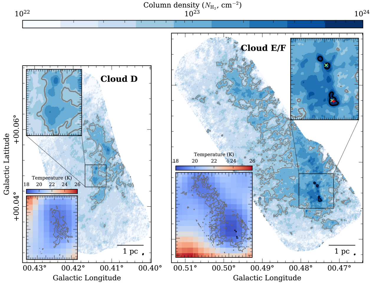
Figure 4. The column density of molecular hydrogen determined towards Cloud D (left-hand panel) and Cloud E/F (right-hand panel). These have been plotted on the same discretized colour scale, and angular size scale for ease of comparison. The grey and black contours overlaid on both panels represent column density levels of N_{\text{H}_2} = [67, 670] \times 10^{21} \text{ cm}^{-2} , respectively (one and two orders of magnitude higher than the star formation relation from Lada et al. 2012, respectively). For clarity, a zoom-in of the core region within Cloud E/F is shown in the upper right of the right-hand panel, overlaid with are red + and green × symbols marking the position of the \text{H}_2\text{O} and \text{CH}_3\text{OH} Class II maser emission, respectively (Caswell et al. 2010; Titmarsh et al. 2016; Lu et al. 2019). Shown in the lower left of the main panels are maps of the Herschel derived dust temperature across each region (Barnes et al. 2017; Battersby et al., in preparation), which were used in the calculation of the column density. The overlaid contours are identical to those in the main panel.
