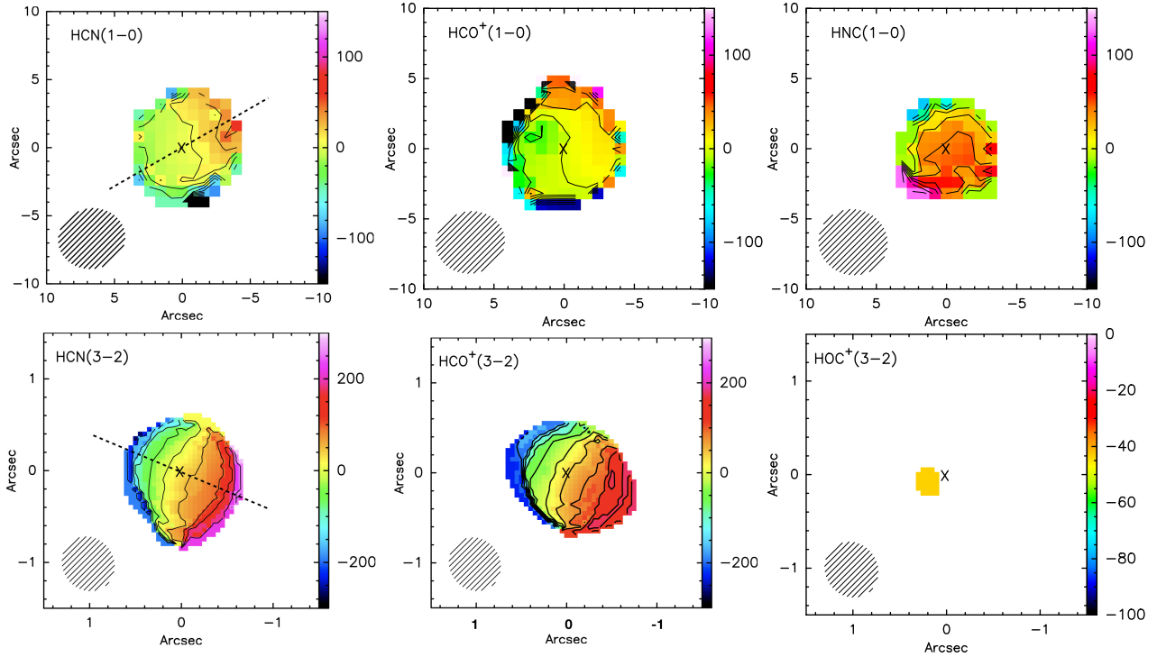
Fig. 8. Velocity fields (moment 1 maps). The coloured velocity scale (right axis) is in \text{km s}^{-1} . The step in contours is 20 \text{ km s}^{-1} for all lines. We note the blue-shifted velocities of \text{HOC}^+(3-2) . The crosses in the centre of each panel indicate the position of the nuclear source. The beam is shown in the lower left corner of each panel. North is up, and east is to the left. The dashed lines in the HCN plots indicate the cut for the p - v diagrams shown in Fig. 9.
