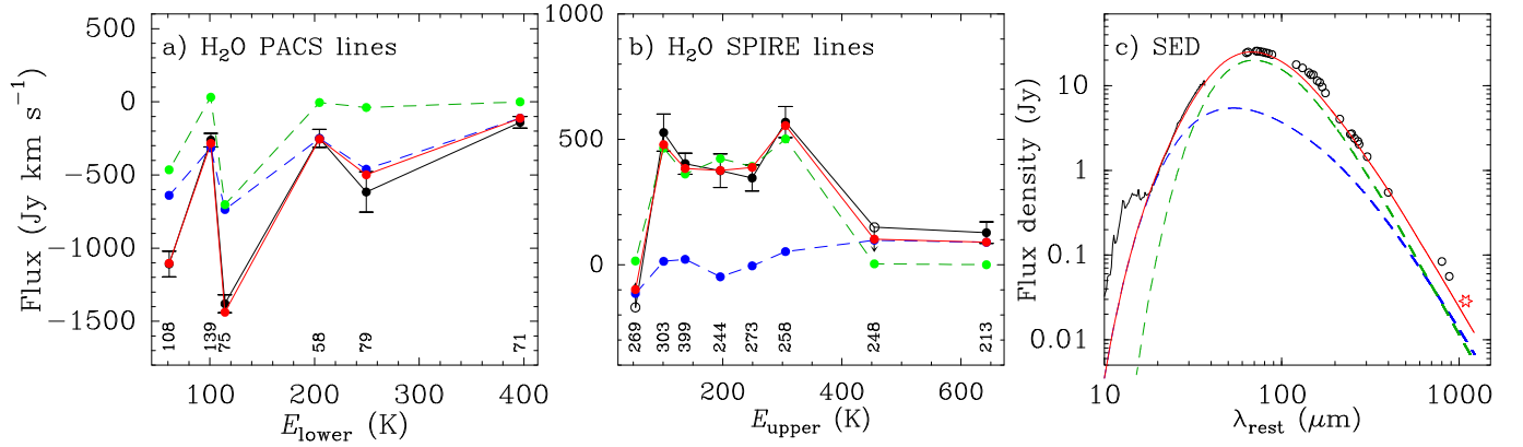
Fig. 15. Comparison between the observed (black symbols) and modelled (coloured symbols and lines) H 2 O fluxes in Mrk 273 within panel a : PACS and panel b : SPIRE. The model includes two components: the core (in blue), which accounts for most absorption lines observed within PACS, and the inner disc (in green), which dominates the emission of the sub-mm lines with E_{\text{upper}} < 400 K observed with SPIRE (see Table 4). Red colours and symbols indicate total modelled fluxes. The numbers at the bottom of panels a and b indicate rounded-up transition wavelengths in \mu\text{m} . Panel c : the SED of Mrk 273, including the Spitzer /IRS spectrum, Herschel /PACS and SPIRE continuum data from observations of both H 2 O and OH lines, sub-mm data at 800 and 880 \mu\text{m} (Rigopoulou et al. 1996; Wilson et al. 2008), and our measured flux density at 1 mm (starred-red symbol), is compared with the prediction of our composite model.
