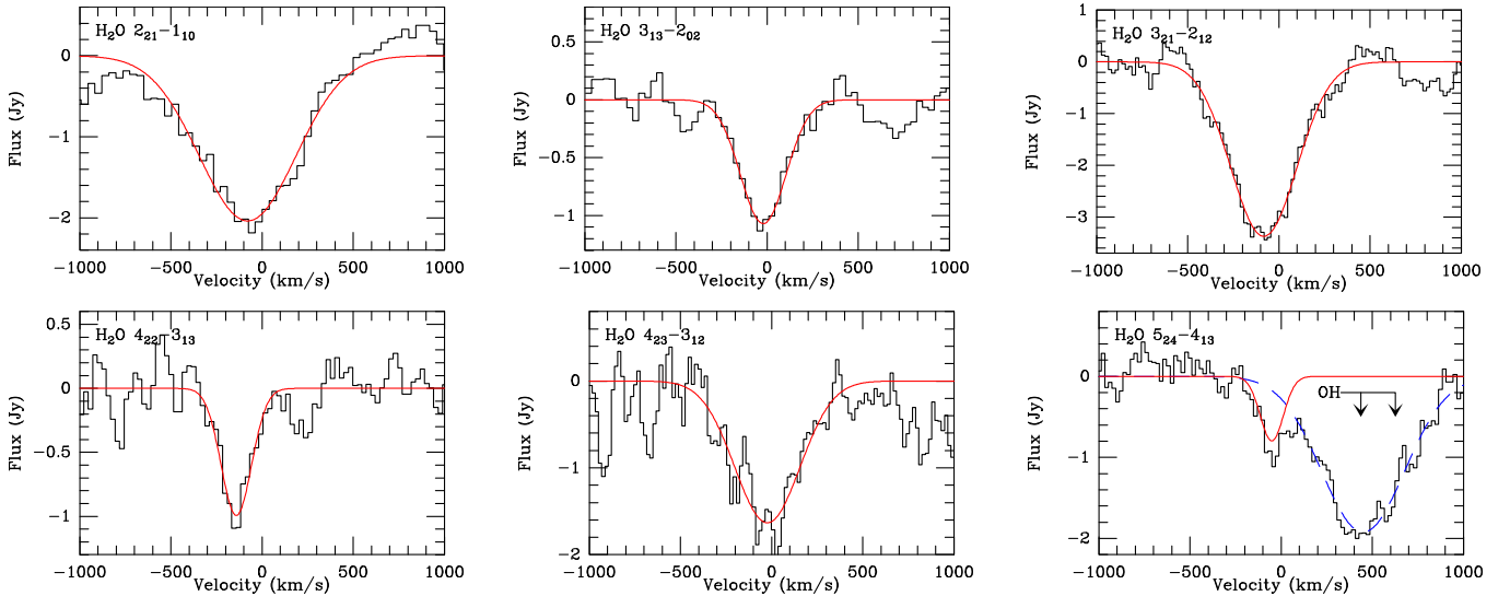
Fig. 3. H 2 O absorption lines (black histograms) detected with Herschel /PACS and Gaussian fits (red lines). The velocity sampling is 20–40 km s -1 .
