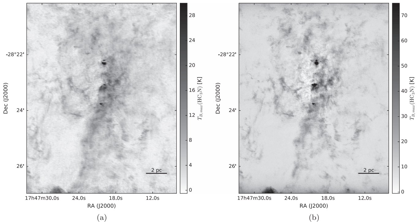
Figure 21. Peak-intensity maps of \text{HC}_3\text{NJ} = 10-9 . The left panel shows the 12 m short-baseline data combined with 7 m and total power data; by excluding the long-baseline data, the large angular scales are emphasized. The right panel shows the robust 0.5-weighted 12 m+7 m data combined with total power data; it reaches a substantially higher peak intensity in the compact regions, but the lower-intensity diffuse emission is relatively hidden. In the right panel, the negative bowls seen near Sgr B2 M and N in this peak-intensity image indicate that intermediate size scales were not well recovered. The bright feature on the lower left of both images may be an imaging artifact.
