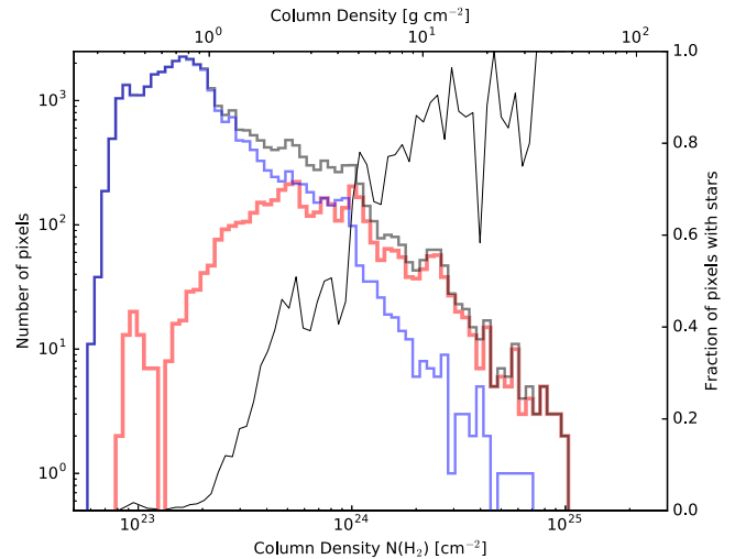
Figure 15. Histograms of the column density measured with the combined SCUBA and Herschel data using the interpolated Herschel temperatures covering only the region observed with ALMA. The black histogram (left axis) shows the whole observed region, the blue solid line shows the SCUBA pixels that do not contain an ALMA source, and the red thick line shows those pixels that are within one beam FWHM of an ALMA source. The thin black line (right axis) shows the ratio of the red histogram to the black histogram, i.e., it shows the fraction of pixels with associated YSOs. While the ALMA sources (high-mass YSOs) clearly reside in high column density gas, there is abundant high column density material that shows no signs of ongoing star formation.
