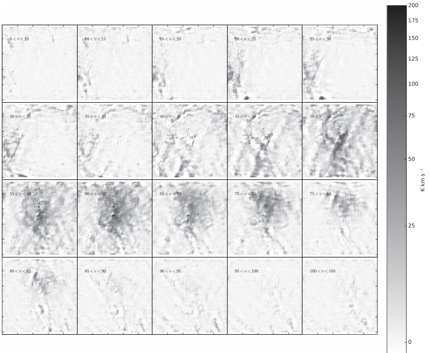
Figure 20. Channel maps of the \text{HC}_3\text{NJ} = 10\text{--}9 line. Each panel shows the integrated intensity over a 5 \text{ km s}^{-1} velocity range as indicated in the figures. The data shown here are 12 \text{ m}+7 \text{ m} images made excluding the long-baseline data sets to emphasize large angular scales combined with total power data by feathering the images. The “ridge” feature discussed in the text is most evident in the 50\text{--}55 \text{ km s}^{-1} channel, and these images show that it is dominated by a single velocity component.
