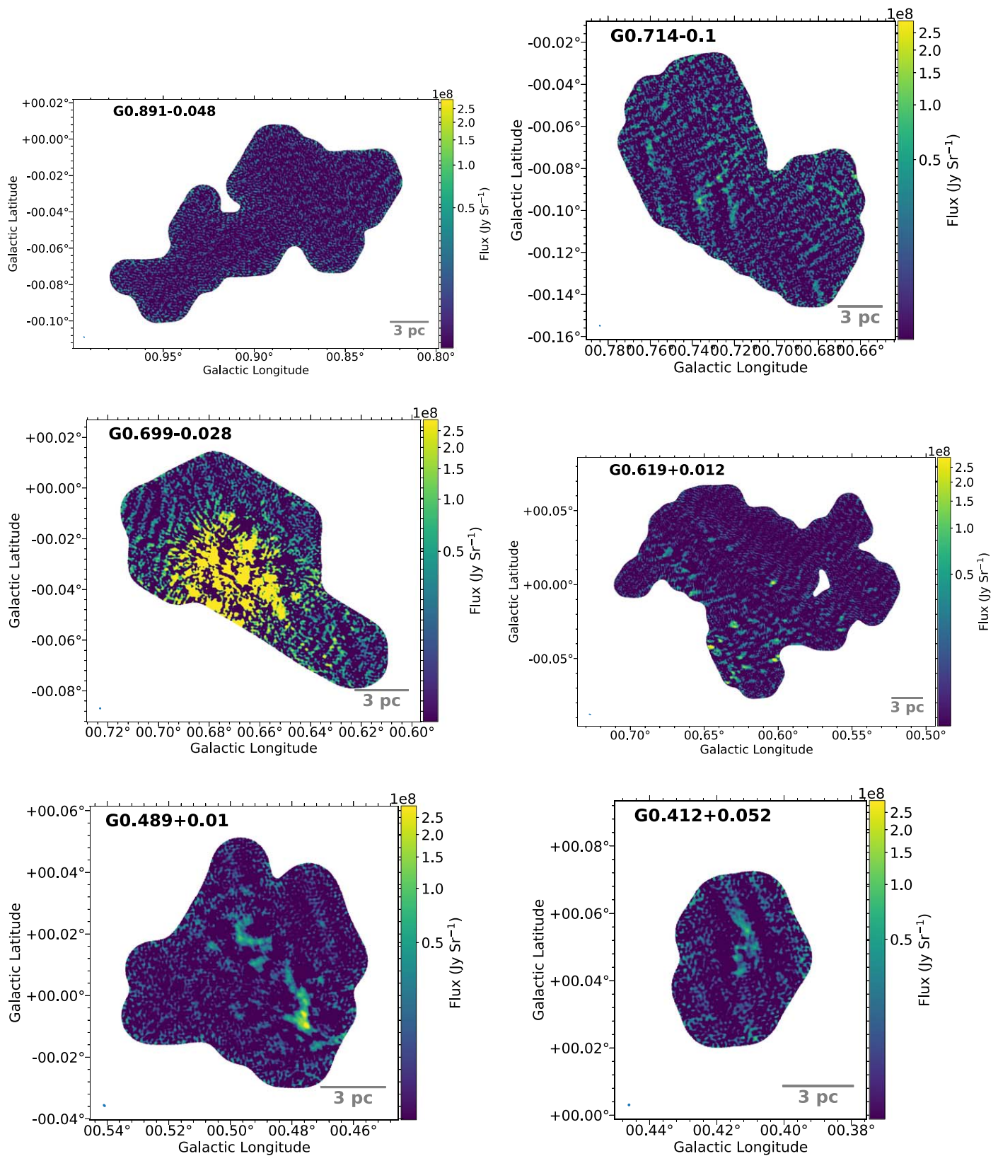
Figure C2. Images of the 1.3 mm dust continuum from the CMZzoom Survey with a 3 pc scale bar. The white contour shows the approximate 5\sigma level while the black contour shows the approximate 10\sigma level. All the images are displayed on same colorscale from 2 to 290 \text{MJy Sr}^{-1} .
