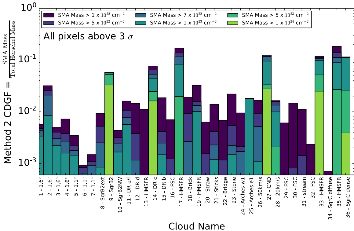
Figure 10. Method 2 CDGF, as measured in a comparison between the SMA and Herschel mass in each cloud. The names on the x-axis consist of a prefix, which is the mask number, and a shorthand name for each cloud, of which more details are provided in Table 2. They are ordered in decreasing central Galactic longitude from left to right. Each bar shows the mass above 3\sigma in the corresponding CMZoom SMA-mapped cloud, above various column density thresholds as shown in the legend, divided by the total mass of the cloud (at all column densities) as seen in Herschel. As also seen in Figure 9, the overall CDGF is less than 10% for most of the clouds, but this figure demonstrates the varying levels of substructure in each cloud. Note that the apparently high CDGF seen toward the CND located near \ell = 0^\circ , is likely due to contamination from the strong synchrotron source Sgr A* and resulting imaging artifacts (see Section 5.4 for more details). The CND is removed from the remaining CDGF plots.
