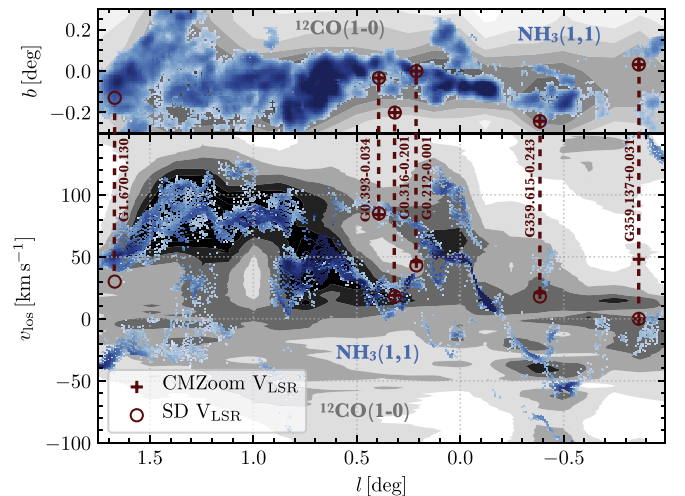
Figure 11. Location of the potential foreground sources, G1.670–0.130, G0.393–0.034, G0.316–0.201, G0.212–0.001, G359.615–0.243, and G359.137+0.031, on a longitude–latitude and longitude–velocity plot of the CMZ. The gray data are CO from Dame et al. (2001) and the color points are the 3D locations of Gaussian fit centroids to NH _3 (1,1) data from The H _2 O Southern Galactic Plane Survey (Walsh et al. 2011; Purcell et al. 2012; Longmore et al. 2017), fit using SCOUSE from Henshaw et al. (2016). The circles indicate the measured peak single-dish velocity of the region and the plus sign indicates the CMZoom preliminary peak velocity of the region as described in detail in Section 5.2 and summarized in Table 3.
