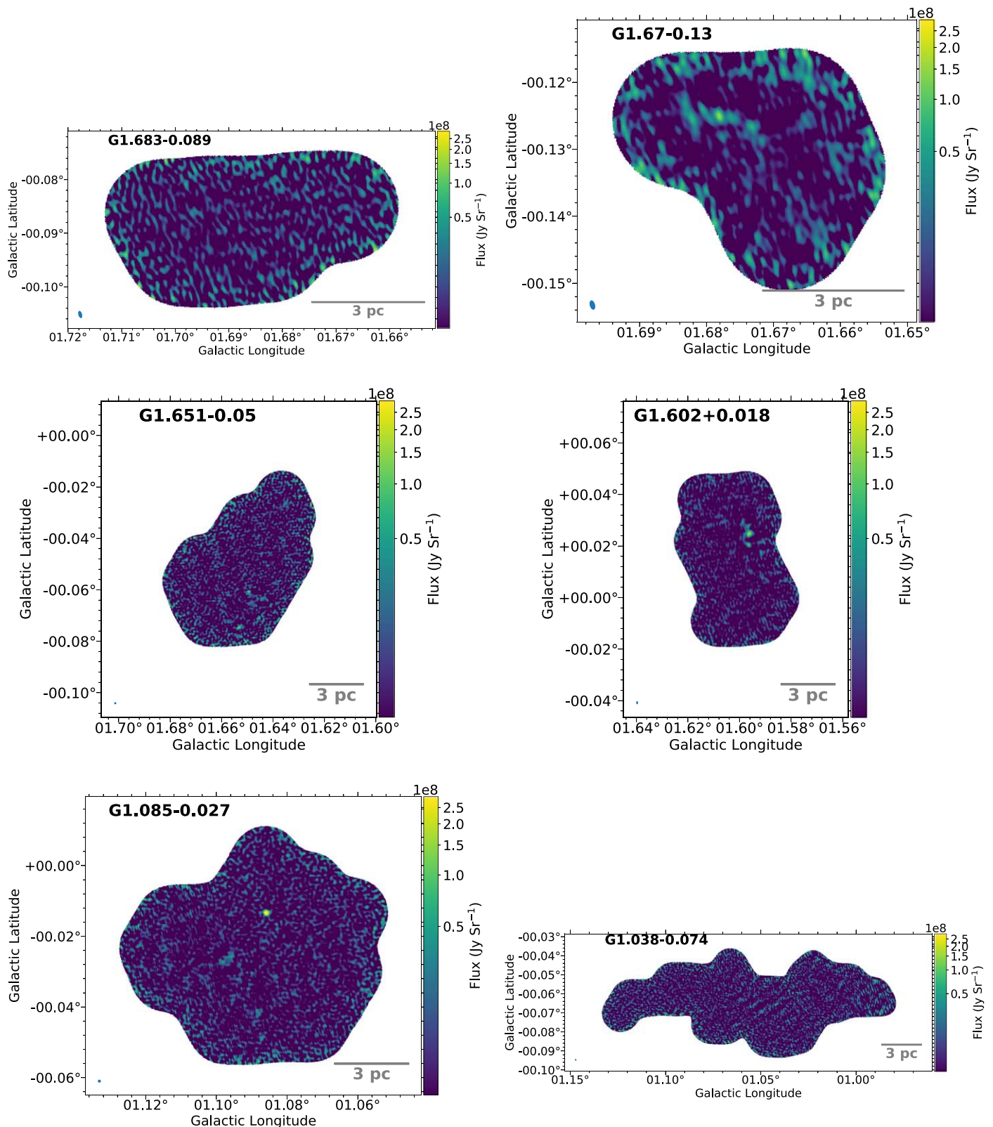
Figure C1. Images of the 1.3 mm dust continuum from the CMZoom Survey with a 3 pc scale bar. The white contour shows the approximate 5\sigma level while the black contour shows the approximate 10\sigma level. All the images are displayed on same colorscale from 2 to 290 \text{ MJy Sr}^{-1} .
