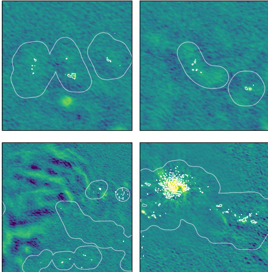
Figure B1. Comparison of CMZoom data with CARMA 3 mm survey from Pound & Yusef-Zadeh (2018). All panels show the CARMA 3 mm dust continuum 15 + 8 (Pound & Yusef-Zadeh 2018), which includes CARMA-15 (the 15-element array with six 10.4 m antennas and nine 6.1 m antennas) as well as CARMA-8 (the eight-element array of 3.5 m antennas) in the same colorscale. The CMZoom survey outline is shown in white. The bottom four figures show zoom-ins on several regions with 5\sigma CMZoom contours (without primary beam correction) in white.
